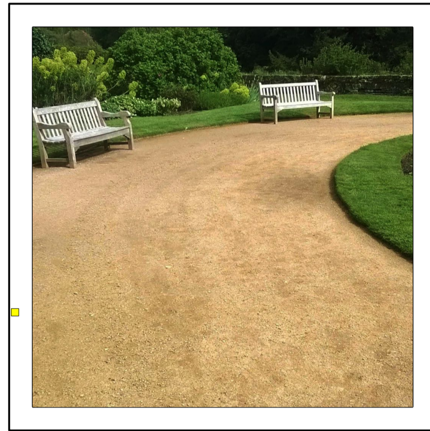
Self binding -Edged with Corten steel. Self binding gravel and Corten steel same level of existing pathways providing step free access.Corten steel provide visual divide between gravel and meadow area.
