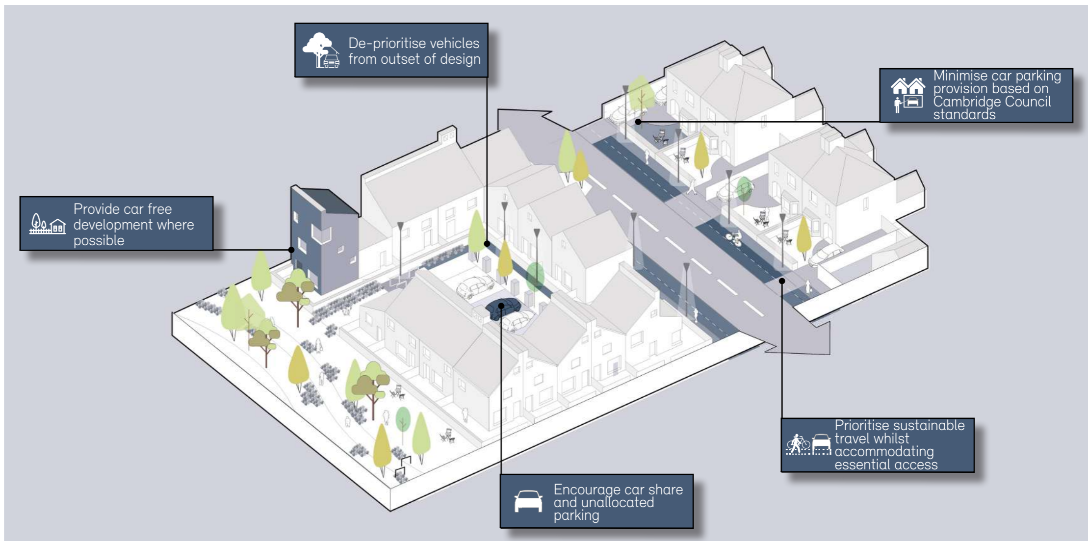
Illustrative diagram showing reducing car dominance principles
